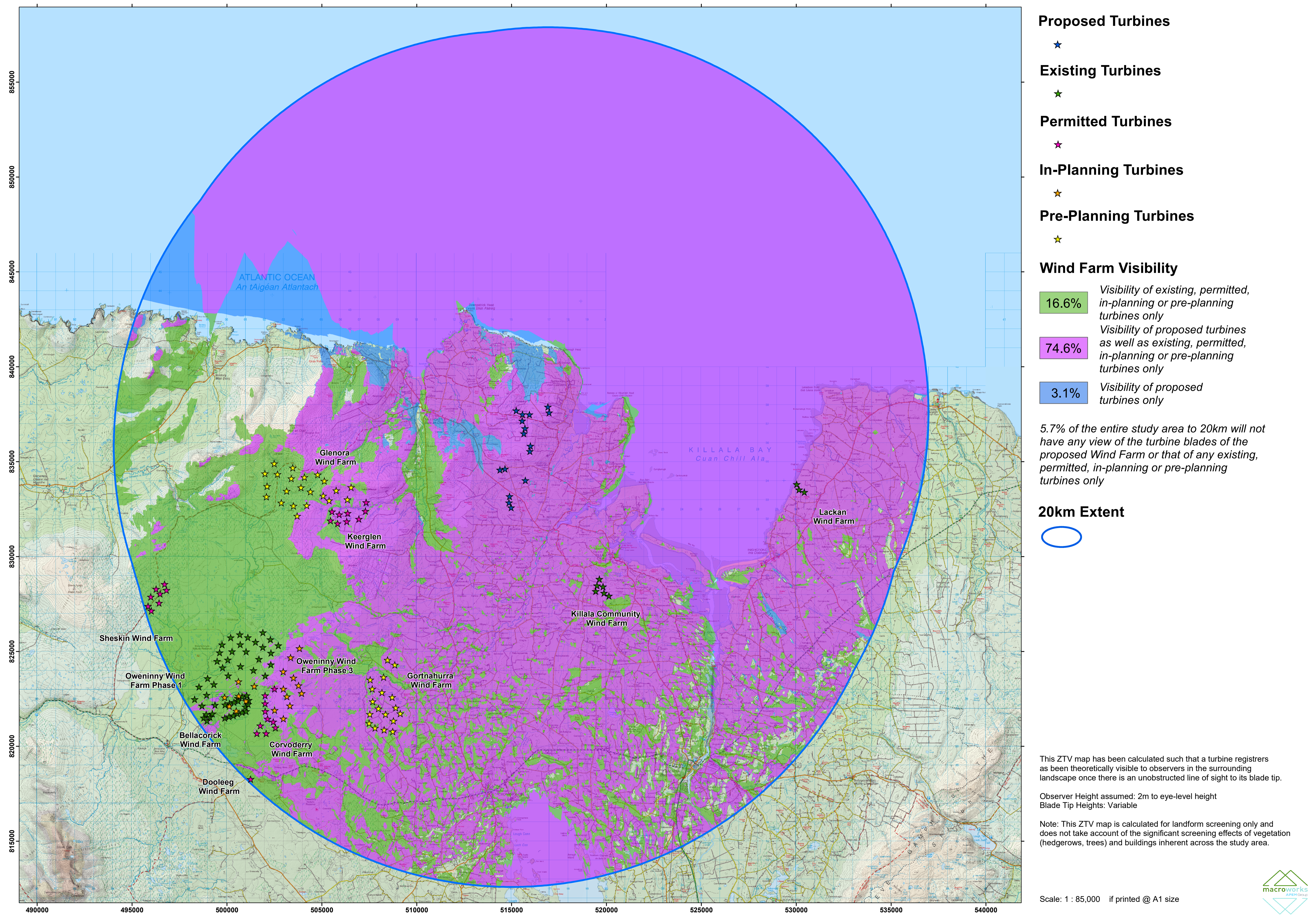
Figure 12.4 ZTV indicating the cumulative theoretical visibility of the proposed Tirawley Wind Farm in combination with the potential future cumulative baseline wind farms in the study area
